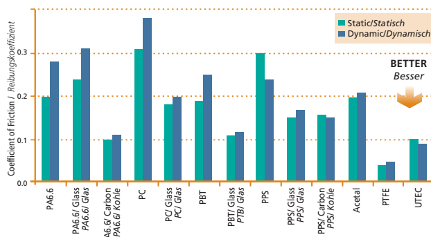
Figure 3 – Static and Dynamic Coefficient of Friction of UTEK and other materials. Data Source: CRAWFORD, R.J. Plastics Engineering. 3 a edição, 1998.
